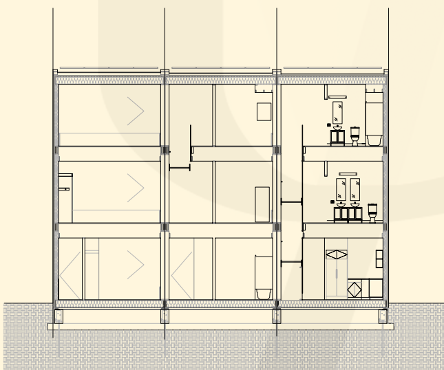
cross section
